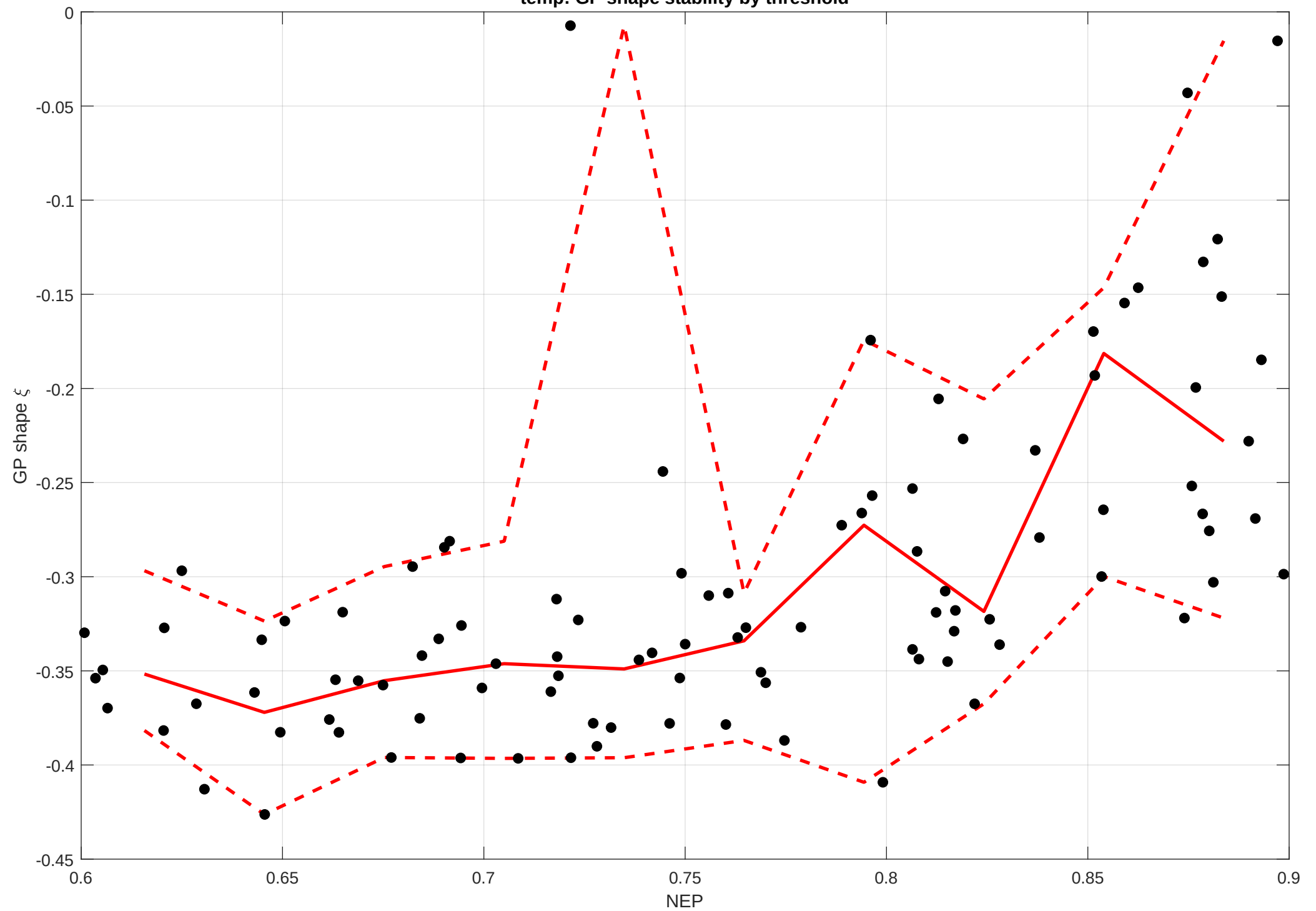
temp: GP shape stability by threshold
